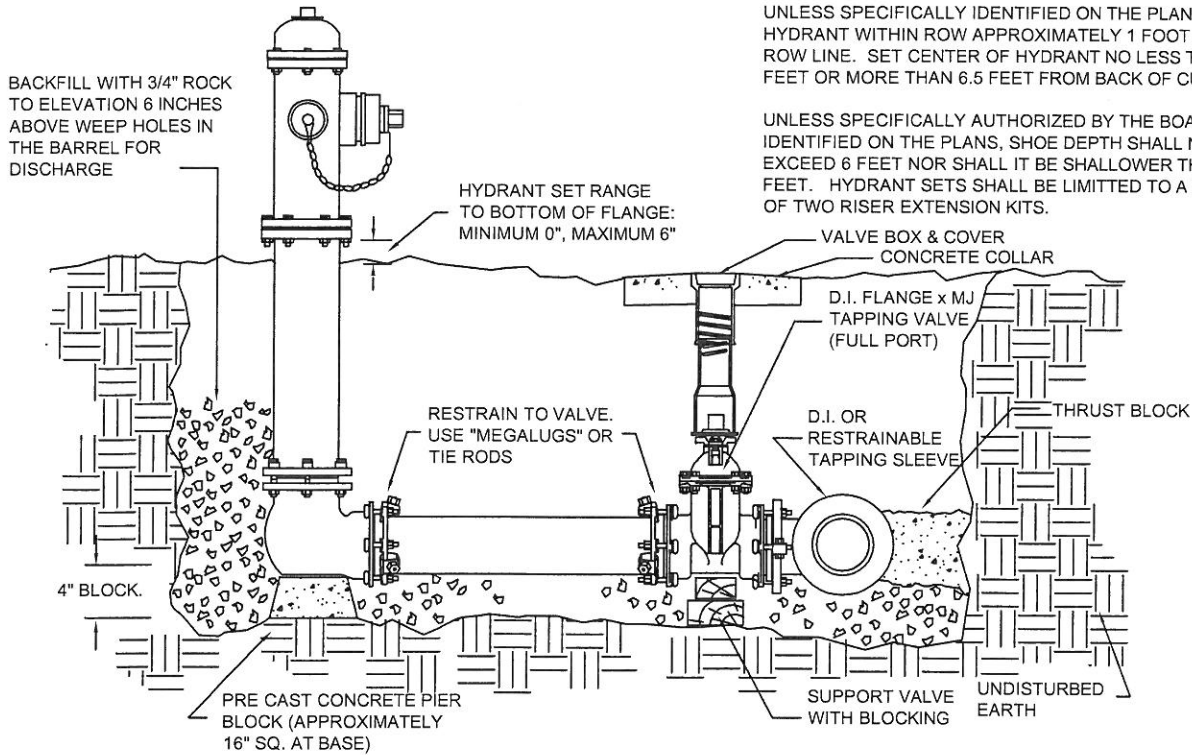
HYDRANT SECTION VIEW
