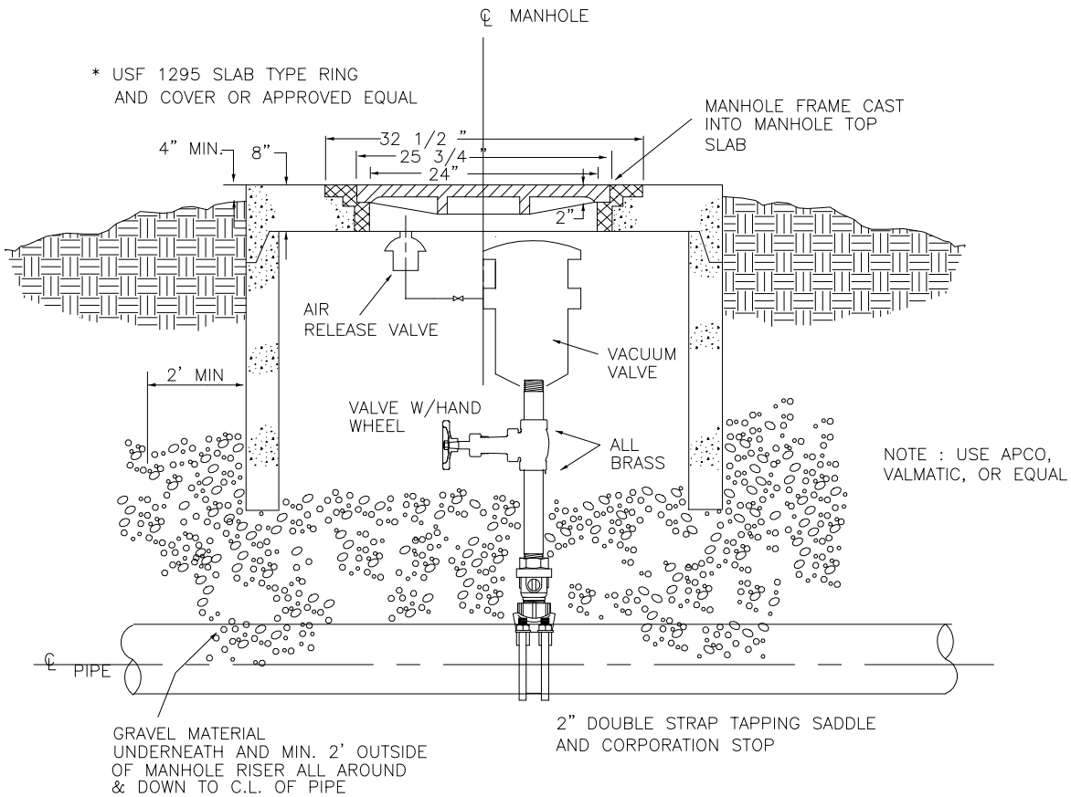
SECTION
