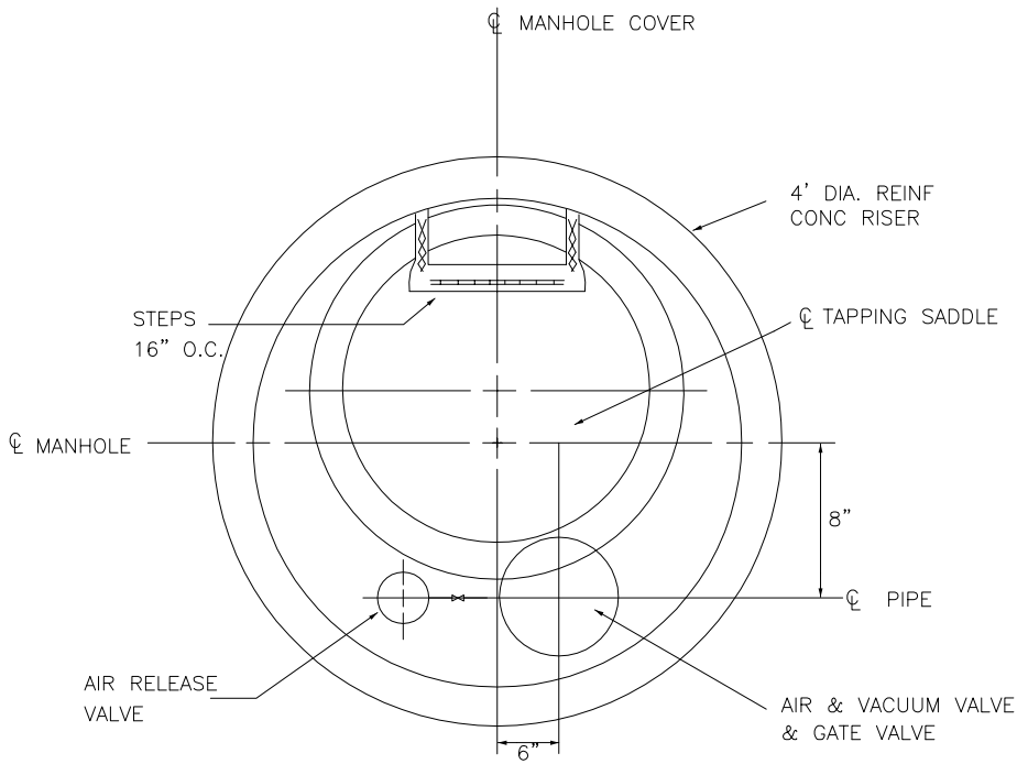
PLAN
