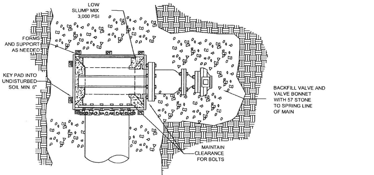
BEVELED GEAR PLAN VIEW
